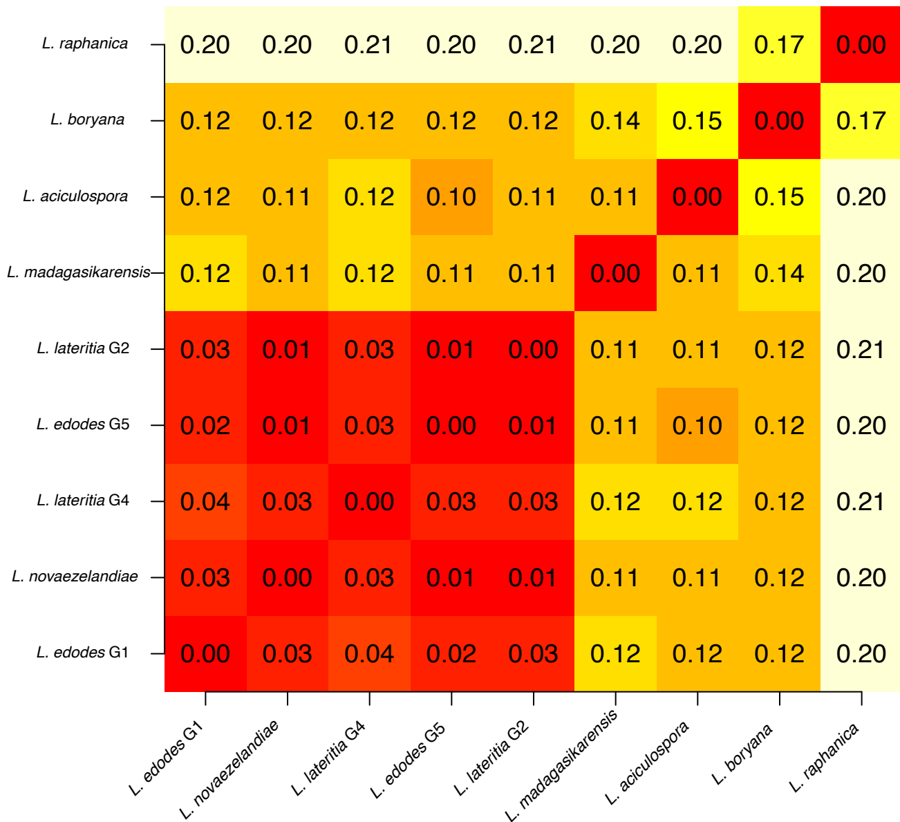
Fig. 3. Distance-matrix heat map of representative sequences of species of Lentinula based on pairwise distances from the ITS multi-sequence alignment given as proportion of divergence.
