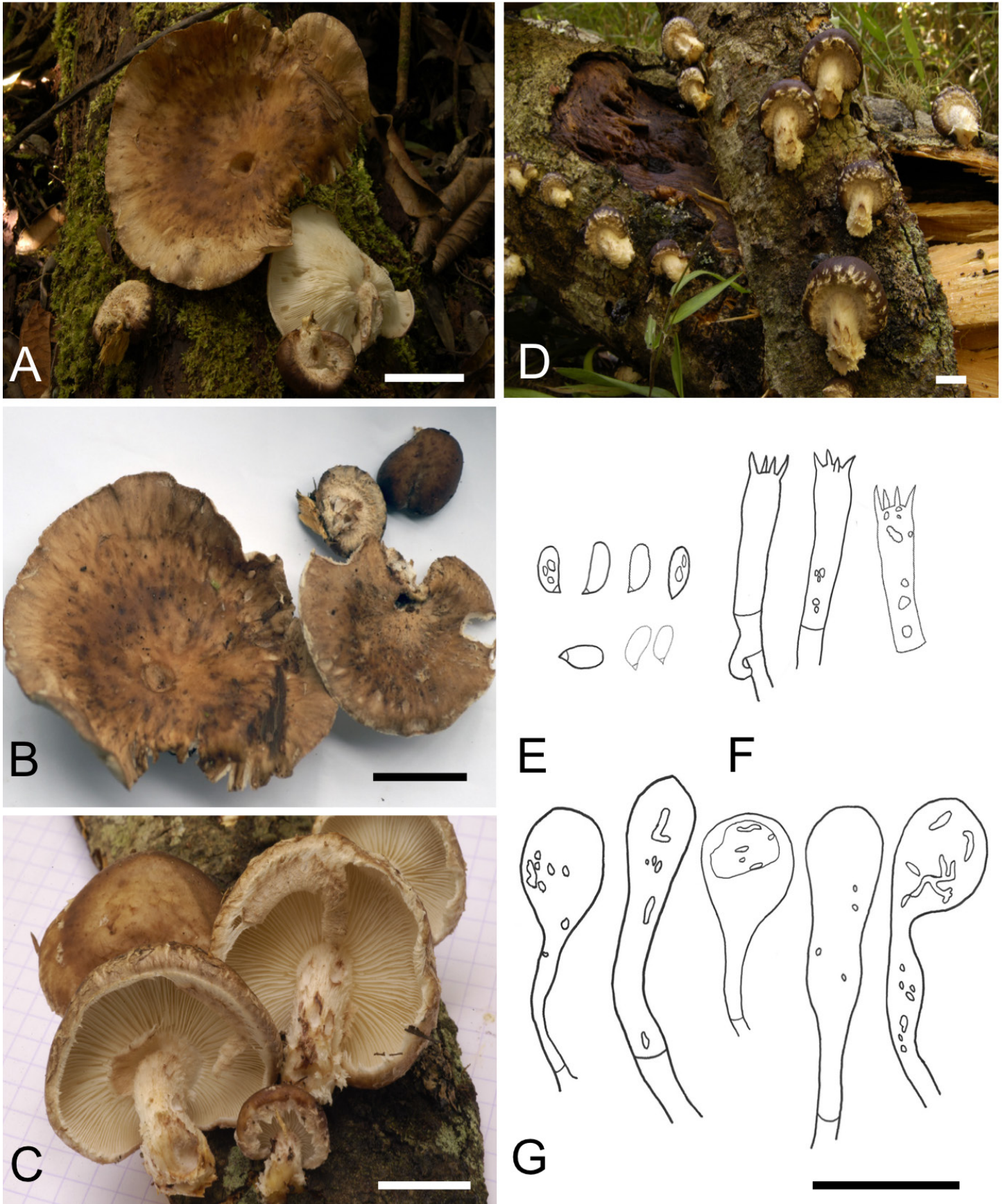
Fig. 4. A, B. Field photograph of Lentinula madagasikarensis (type specimen, PC coll. BB06.007). C, D. Field photographs of Lentinula madagasikarensis (paratype specimen, PC coll. BB08.120). E. Basidiospores. F. Basidia. G. Cheilocystidia. Scale bars: A–D = 2 cm, E–G = 20 \mu m.
