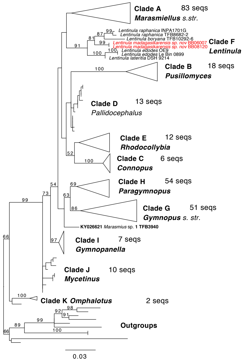
Fig. 1. Maximum-likelihood phylogeny of Omphalotaceae based on the 28S sequence dataset of Oliveira et al. (2019) with 788 bootstrap replicates according to autoMRE bootstopping criteria. Major clades from the original study are labeled and collapsed with number of samples included in each clade. BS values \geq 50\% are included with the branches.
