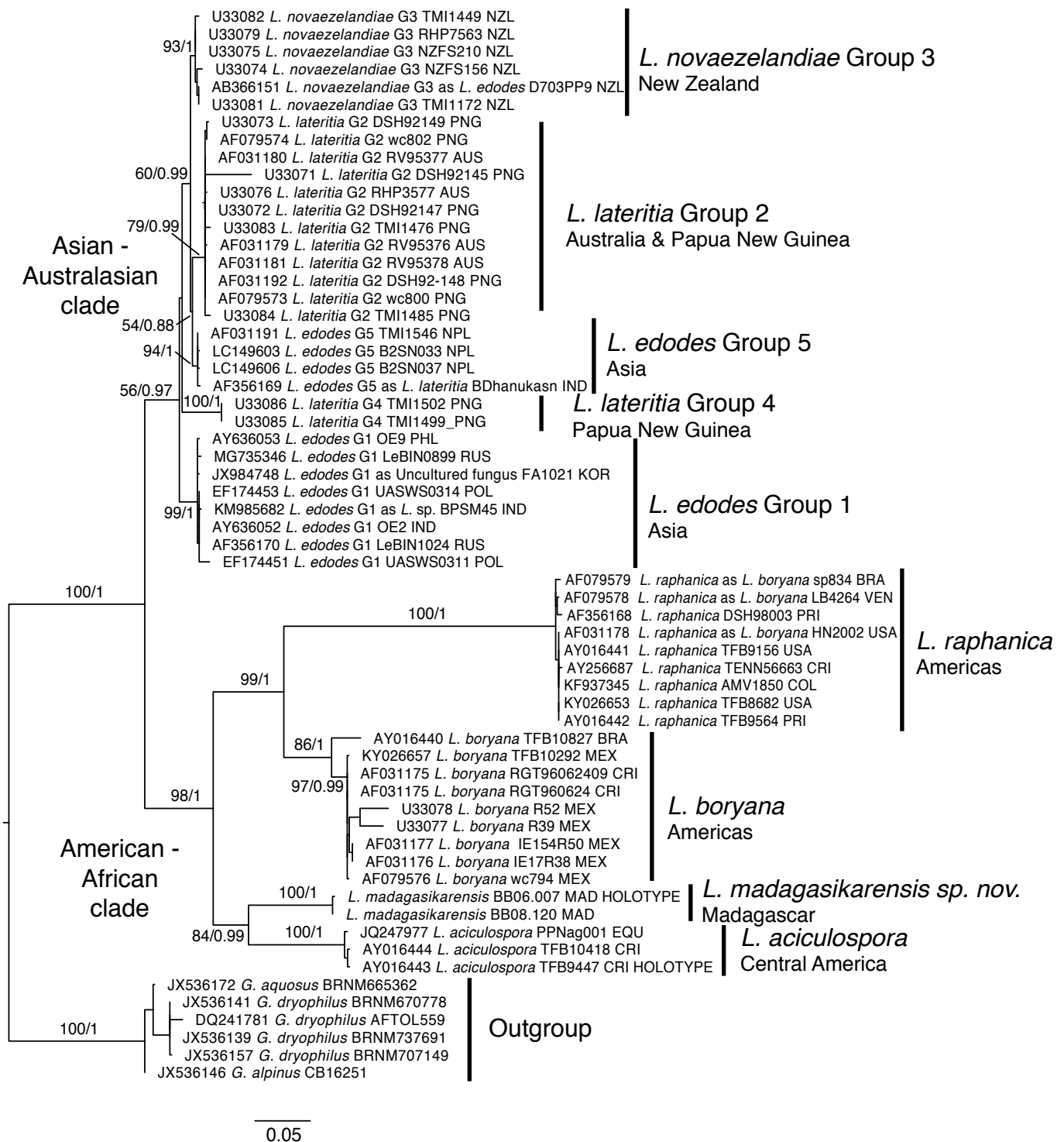
Fig. 2. Maximum-likelihood phylogeny of Lentinula based on Dataset 2 of ITS. BS values \geq 50\% / Bayesian PP values \geq 0.80 are included with the branches. Sequence labels include GenBank accession numbers and collection numbers. G1–G5 in the Asian-Australasian clade correspond to ITS-based groups from Hibbett et al. (1998). Country codes: AUS = Australia, BRA = Brazil, COL = Colombia, CRI = Costa Rica, IND = India, KOR = South Korea, MEX = Mexico, NPL = Nepal, NZL = New Zealand, PHL = Philippines, PNG = Papua New Guinea, POL = Poland (possible cultivar), PRI = Puerto Rico, RUS = Russia, USA = continental USA, VEN = Venezuela.
