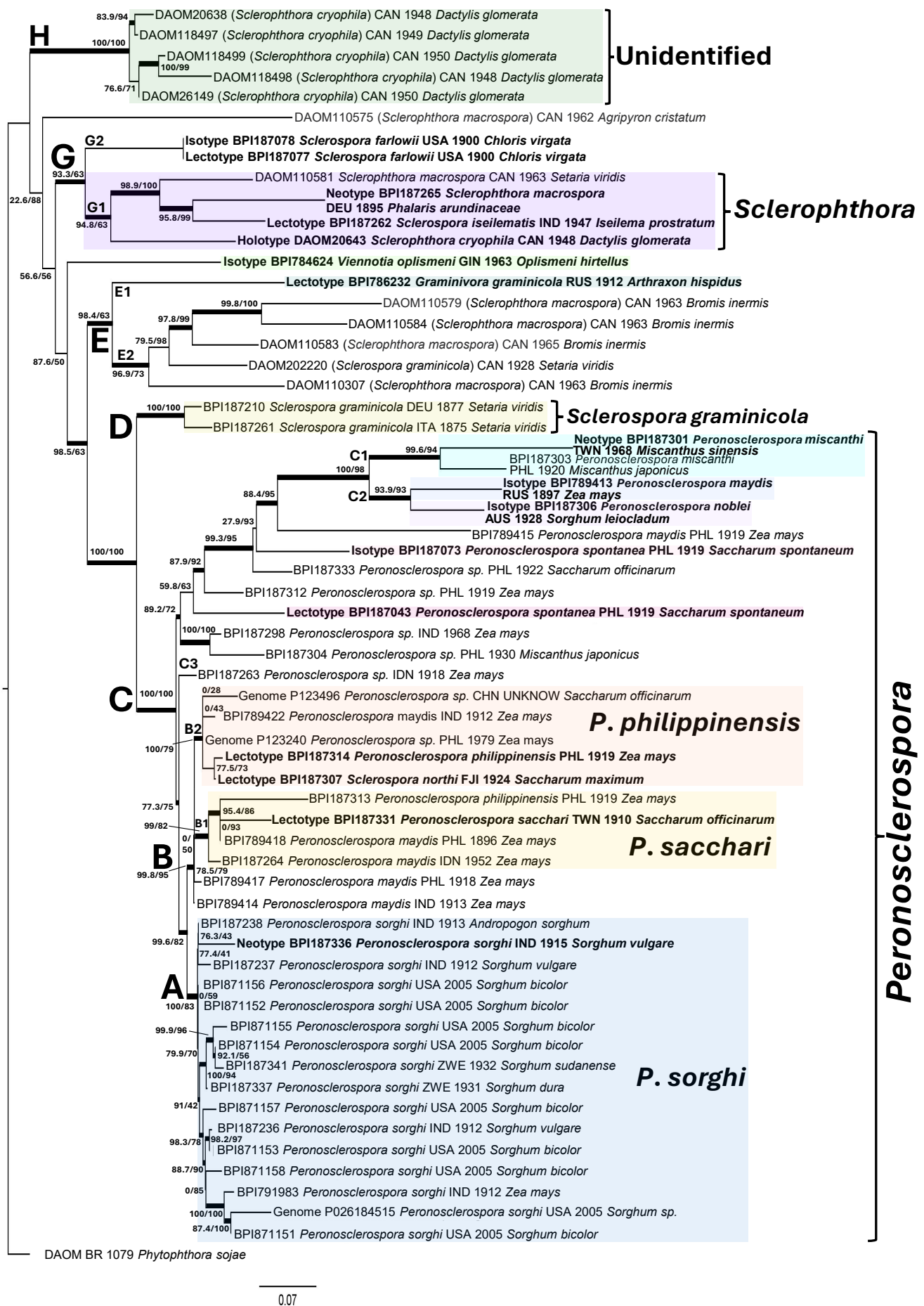
Fig. 1. Maximum likelihood phylogenetic tree computed from 62 filtered, trimmed, and concatenated ortholog sequences. The tree was outgroup rooted to Phytophthora sojae . Bootstraps are displayed on the branches as approximate likelihood ratio test Shimodaira–Hasegawa/ultrafast bootstrap values.
